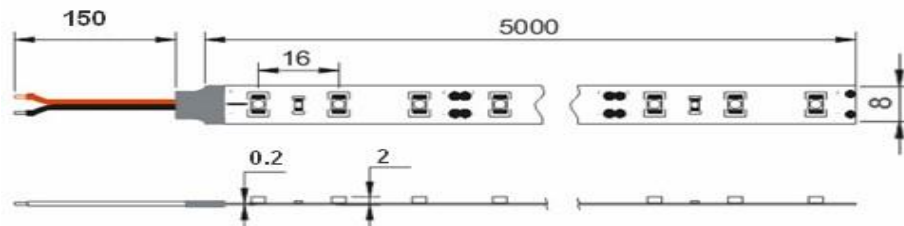
Dimension Drawings (60LED/m)
