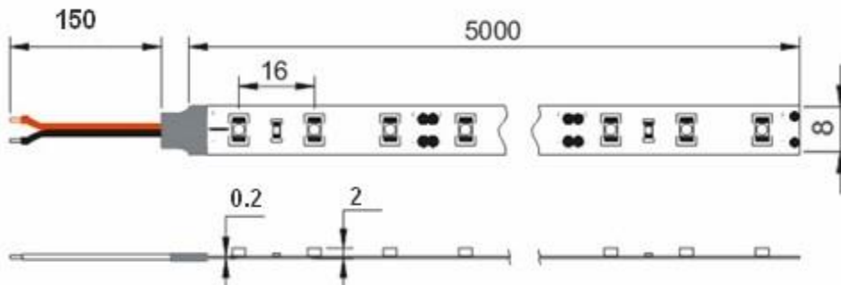
Dimension Drawings (60LED/m)
