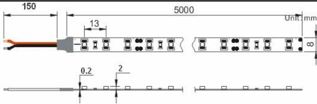
Dimension Drawings (60LED/m)
